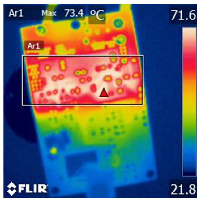
Figure 44 – 120 VAC 60 Hz, 250 W Synthetic Low PF Load, Bottom.
