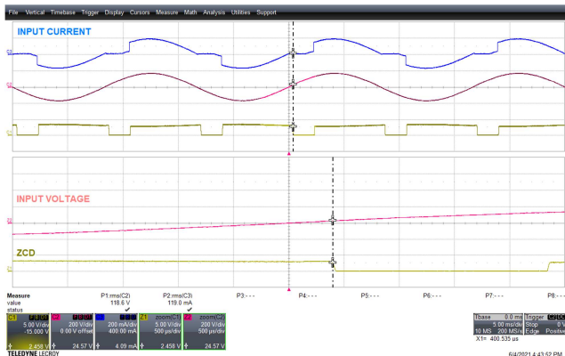
Figure 39 – 120 VAC 60 Hz. CH1: ZCD, 5 V / div., 5 ms / div. CH2: V_{\text{IN}} , 200 V / div., 5 ms / div. CH3: I_{\text{IN}} , 200 mA / div., 5 ms / div. Falling-edge Delay: 400 \mu\text{s} .
