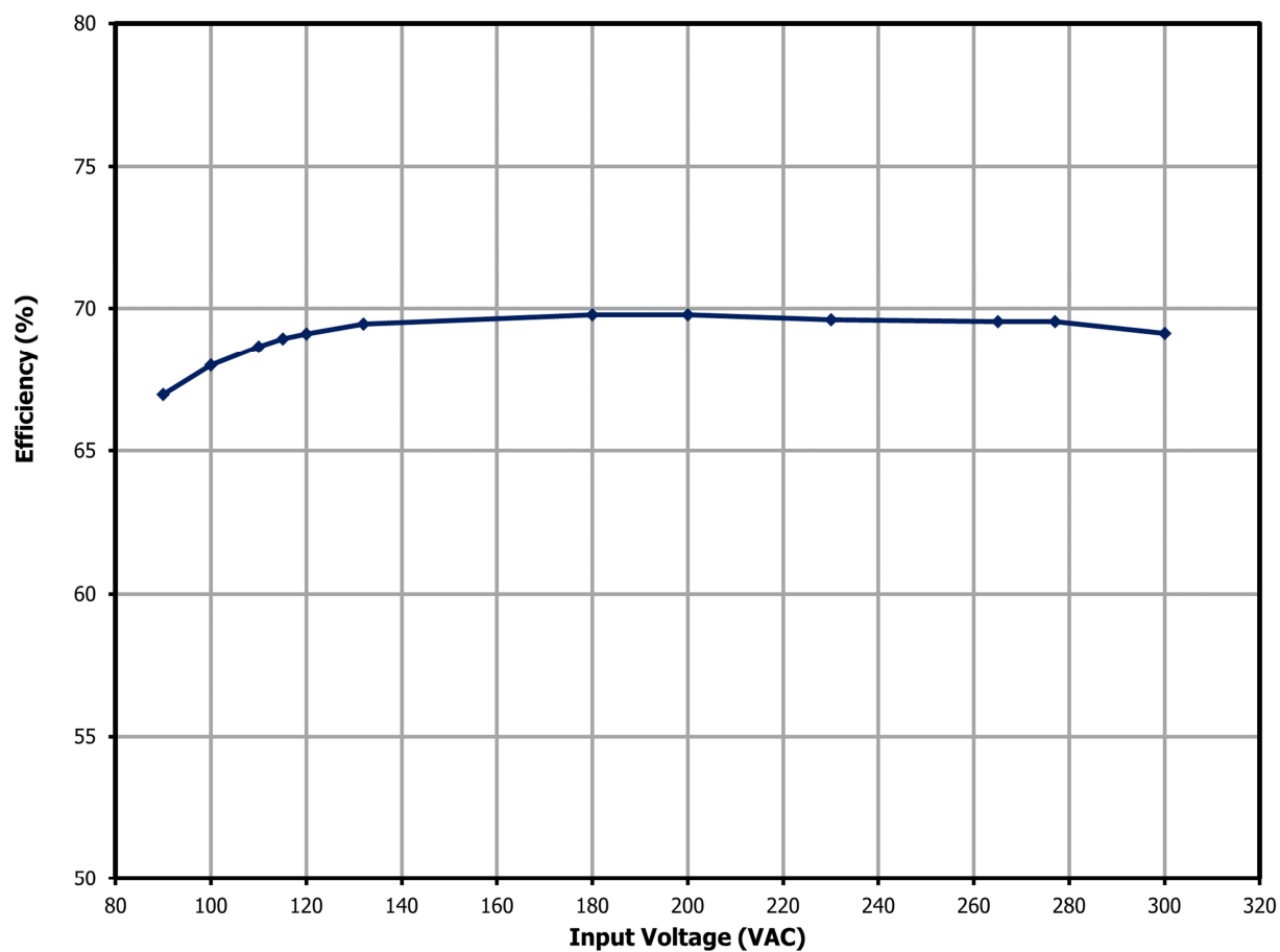
Figure 12 – Full Load Efficiency vs. Line.
