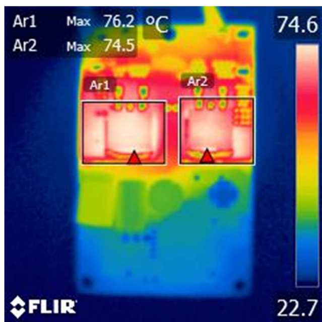
Figure 43 – 120 VAC 60 Hz, 250 W Synthetic Low PF Load, Top.
