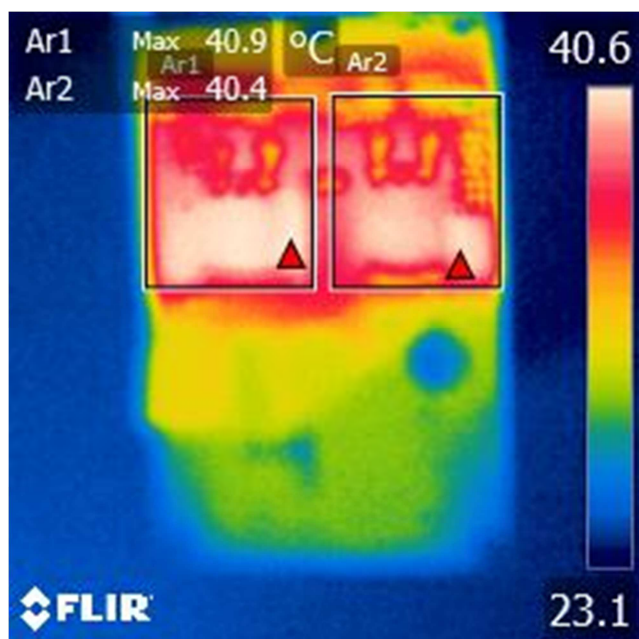
Figure 45 – 120 VAC 60 Hz, 500 W Synthetic High-PF Load, Top.
