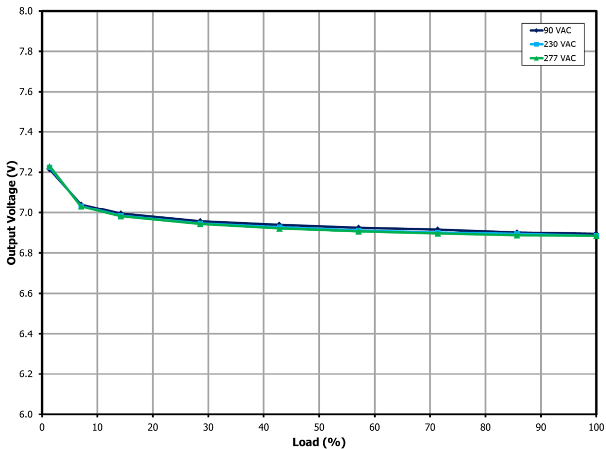
Figure 15 – Output Voltage vs. Percent Load.
