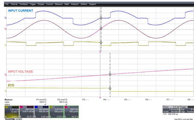
Figure 40 – 230 VAC 50 Hz. CH1: ZCD, 5 V / div., 5 ms / div. CH2: V_{\text{IN}} , 200 V / div., 5 ms / div. CH3: I_{\text{IN}} , 200 mA / div., 5 ms / div. Falling-edge Delay: 266 \mu\text{s} .
