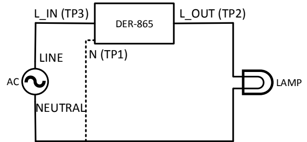
Figure 5 – 3-Wire Connection Diagram.
