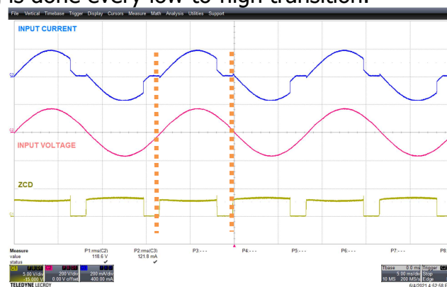
Figure 8 – Trailing-Edge Mode ZCD Detection.
