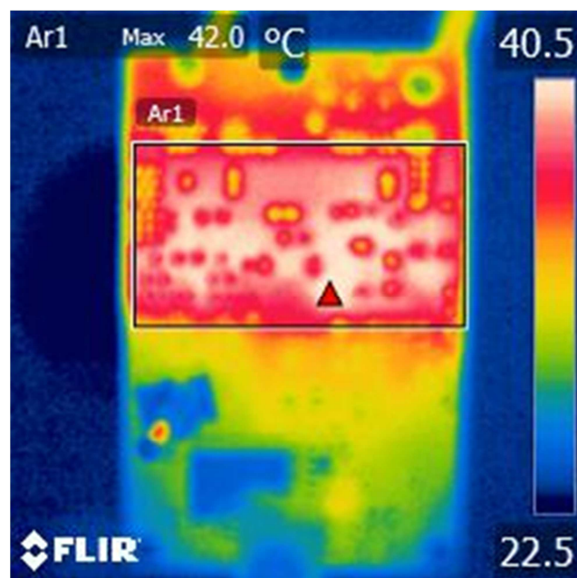
Figure 46 – 120 VAC 60 Hz, 500 W Synthetic High-PF Load, Bottom.
