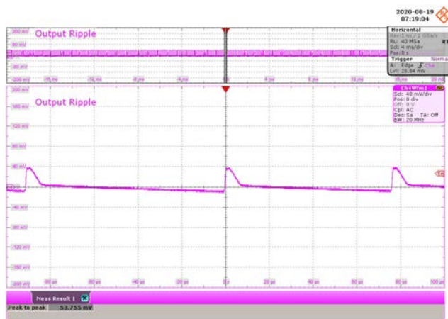
Figure 127 – 90 VAC 60 Hz.
