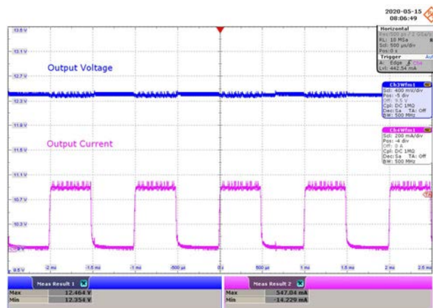
Figure 46 – 300 VAC 50 Hz.
