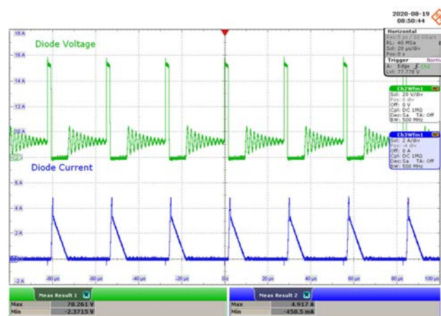
Figure 86 – 300 VAC 50 Hz.
