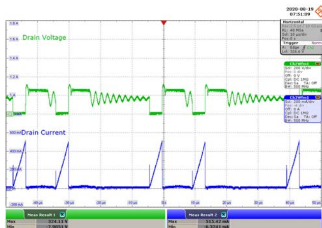
Figure 68 – 115 VAC 60 Hz.
