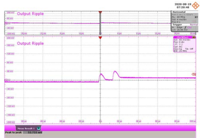
Figure 132 – 115 VAC 60 Hz.
