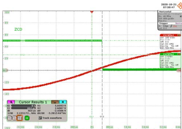
Figure 39 – 115 VAC 60 Hz.
