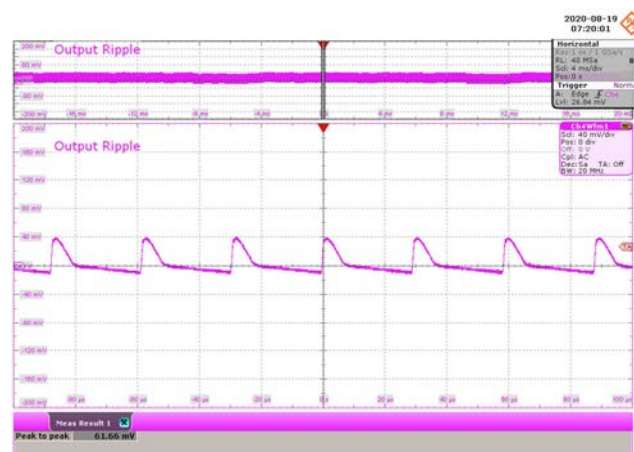
Figure 120 – 115 VAC 60 Hz.
