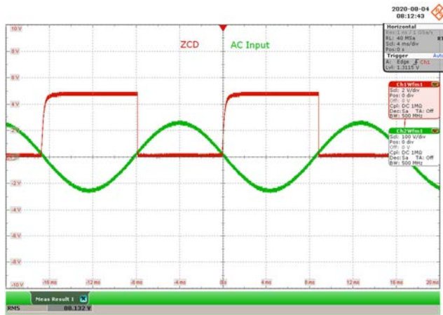
Figure 15 – 90 VAC 60 Hz.
