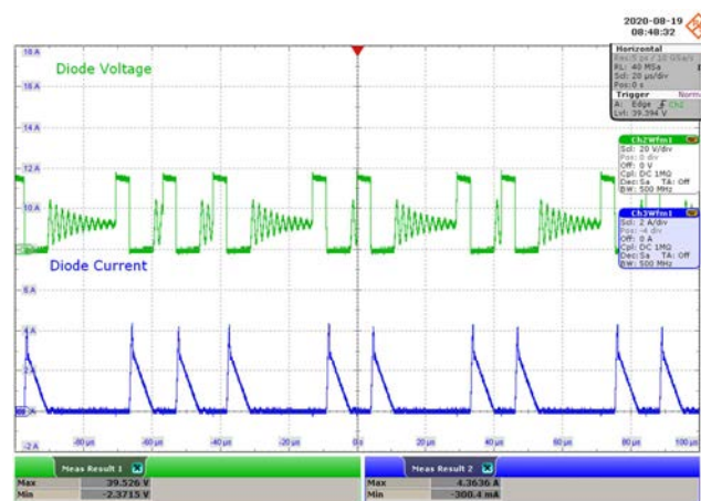
Figure 84 – 115 VAC 60 Hz.
