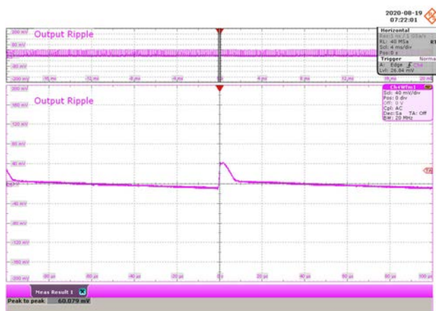
Figure 129 – 230 VAC 50 Hz.
