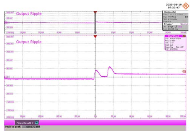
Figure 134 – 300 VAC 50 Hz.
