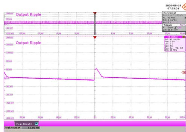
Figure 130 – 300 VAC 50 Hz.
