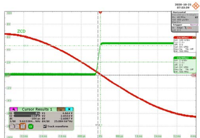
Figure 42 – 230 VAC 50 Hz.
