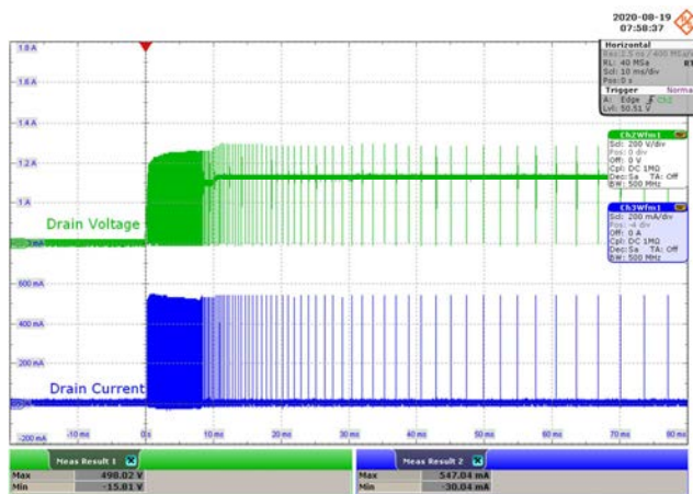
Figure 81 – 230 VAC 50 Hz.
