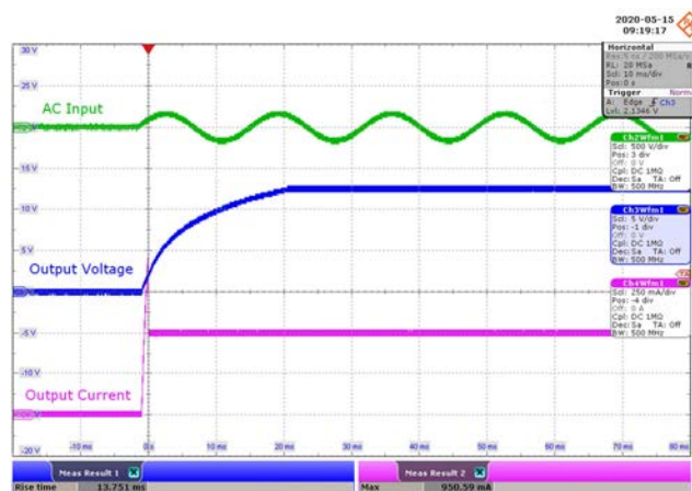
Figure 52 – 115 VAC 60 Hz.
