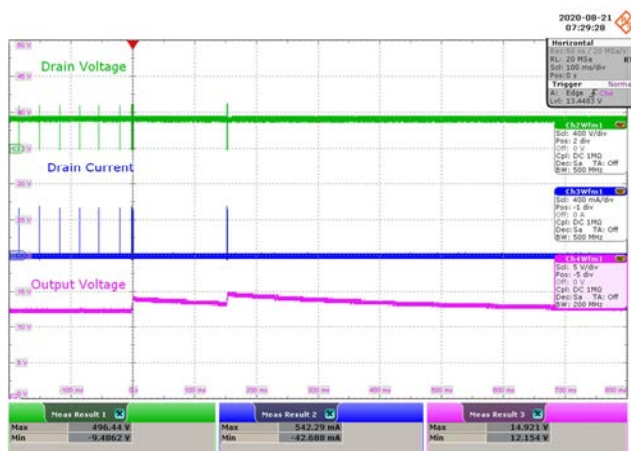
Figure 109 – 230 VAC 50 Hz.
