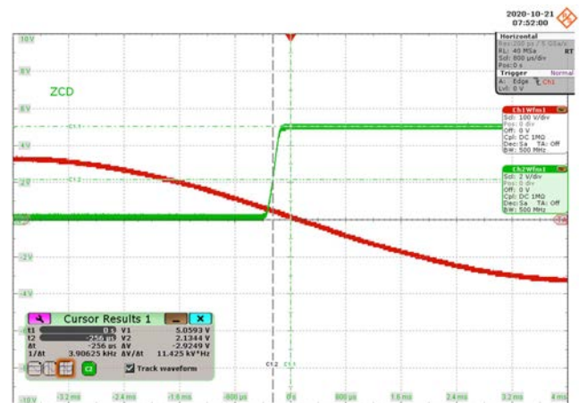
Figure 40 – 115 VAC 60 Hz.
