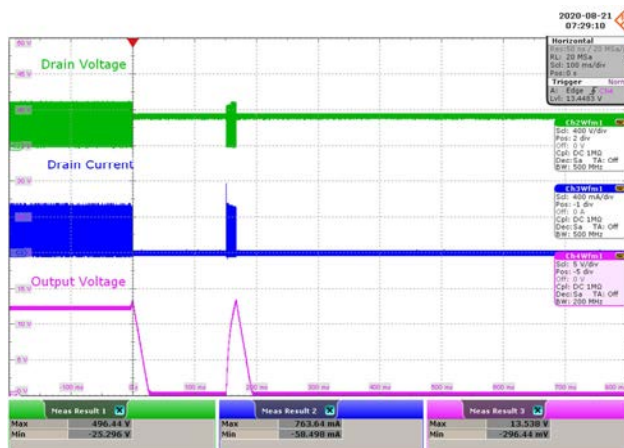
Figure 105 – 230 VAC 50 Hz.
