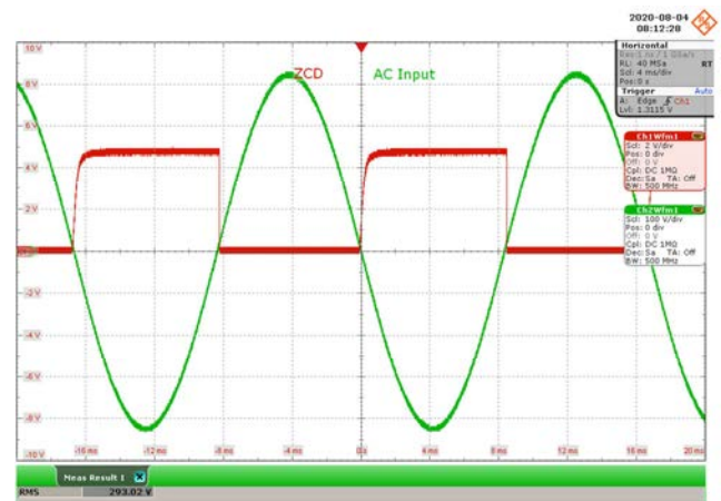
Figure 18 – 300 VAC 50 Hz.
