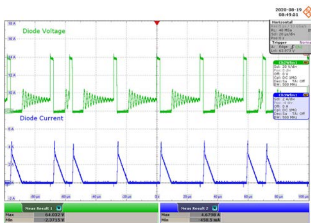
Figure 85 – 230 VAC 50 Hz.
