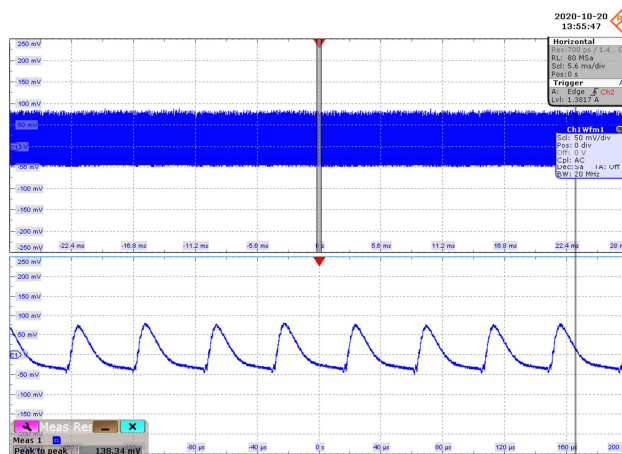
Figure 49 – Output Voltage Ripple.
