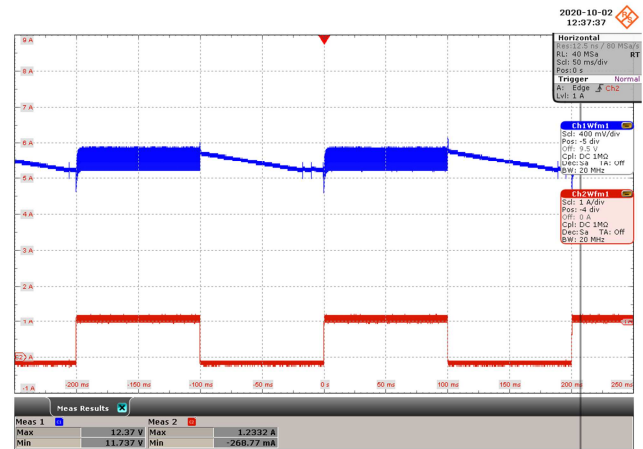
Figure 68 – Output Load Transient, 100 % to 0 % Load.
