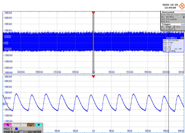
Figure 40 – Output Voltage Ripple.
