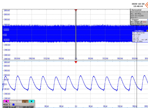
Figure 41 – Output Voltage Ripple.
