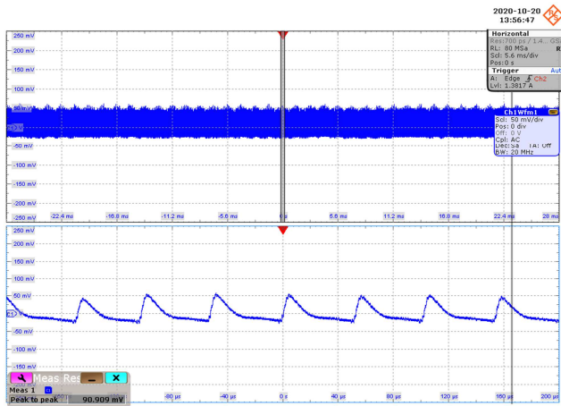
Figure 52 – Output Voltage Ripple.
