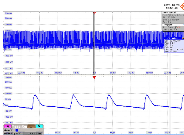
Figure 51 – Output Voltage Ripple.
