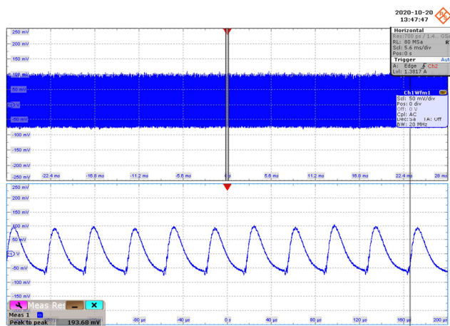
Figure 42 – Output Voltage Ripple.
