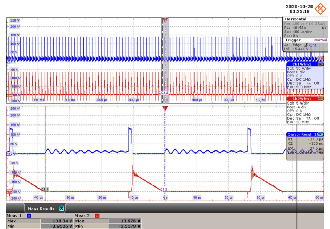
Figure 33 – SRFET Drain to Source Voltage Waveforms. V_{IN} = 1200 \text{ VDC} , I_{OUT} = 1.25 \text{ A} . SRFET V_{DS(MAX)} = 138.3 V. SRFET I_{DS(MAX)} = 13.7 A. Upper: SRFET V_{DS} , 50 V, 400 \mu\text{s} / div. Lower: SRFET I_{DS} , 5 A, 400 \mu\text{s} / div. Bottom Half: Zoom @ 10 \mu\text{s} / div.
