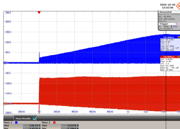
Figure 37 – SRFET Drain to Source Voltage Waveforms.
