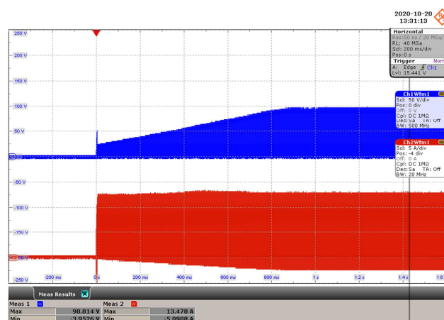
Figure 35 – SRFET Drain to Source Voltage Waveforms.
