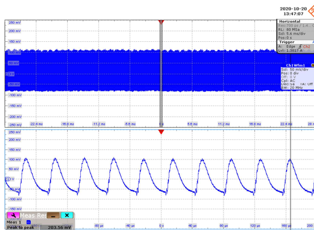
Figure 43 – Output Voltage Ripple.
