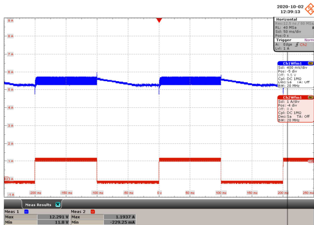
Figure 65 – Output Load Transient, 100% to 0% Load.
