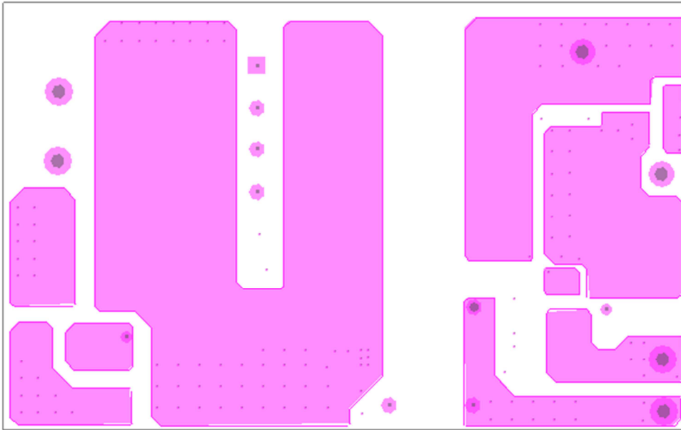
Figure 6 – Printed Circuit Board Layout (Internal layer 1).
