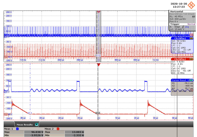
Figure 31 – SRFET Drain to Source Voltage Waveforms. V_{IN} = 800 \text{ VDC} , I_{OUT} = 1.25 \text{ A} . SRFET V_{DS(MAX)} = 96.8 V. SRFET I_{DS(MAX)} = 13.1 A. Upper: SRFET V_{DS} , 50 V, 400 \mu\text{s} / div. Lower: SRFET I_{DS} , 5 A, 400 \mu\text{s} / div. Bottom Half: Zoom @ 10 \mu\text{s} / div.
