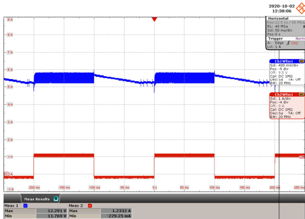
Figure 67 – Output Load Transient, 100% to 0% Load.
