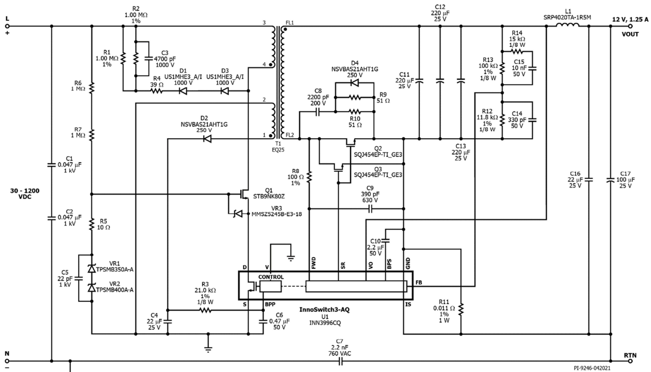
Figure 3 – Schematic.
