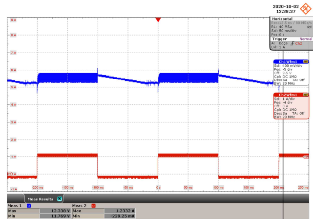
Figure 66 – Output Load Transient, 100 % to 0 % Load.
