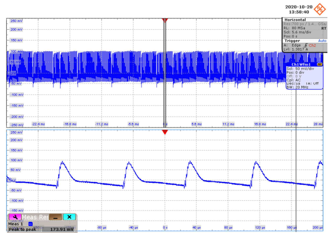
Figure 55 – Output Voltage Ripple.
