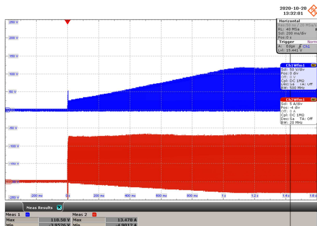
Figure 36 – SRFET Drain to Source Voltage Waveforms.
