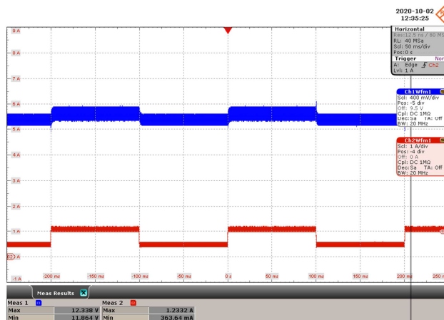
Figure 62 – Output Load Transient, 100 % to 50 % Load. V_{IN} = 800 VDC, I_{OUT} = 1.25 A to 0.625 A. V_{OUT(MAX)} = 12.34 V, V_{OUT(MIN)} = 11.85 V. Upper: V_{OUT} , 400 mV, 50 ms / div. Lower: I_{OUT} , 1 A, 50 ms / div.
