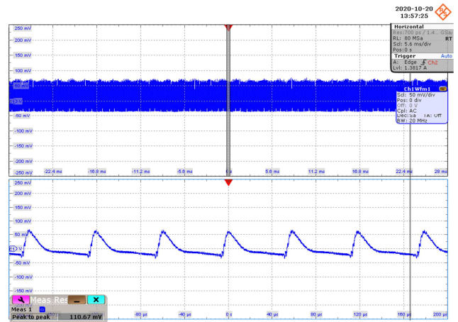
Figure 53 – Output Voltage Ripple.
