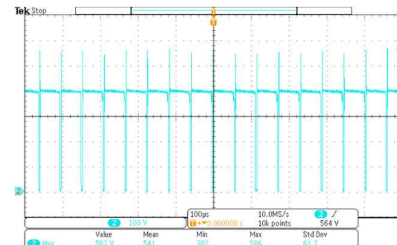
264Vac Operating Short Vds(max) : 562V
