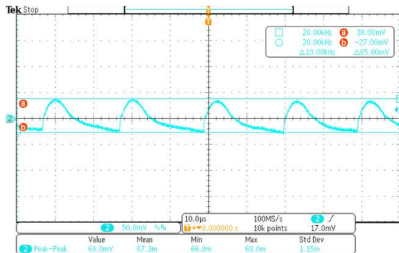
230Vac Full Load Ripple: 68mV
