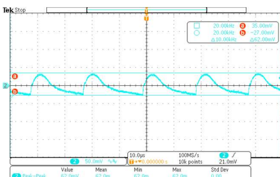
264Vac Full Load Ripple: 62mV
