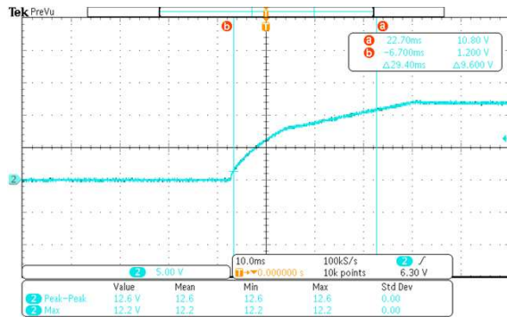
90Vac Rise Time: 29.4mS
