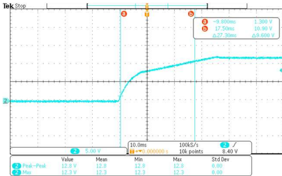
230Vac Rise Time: 27.3mS
