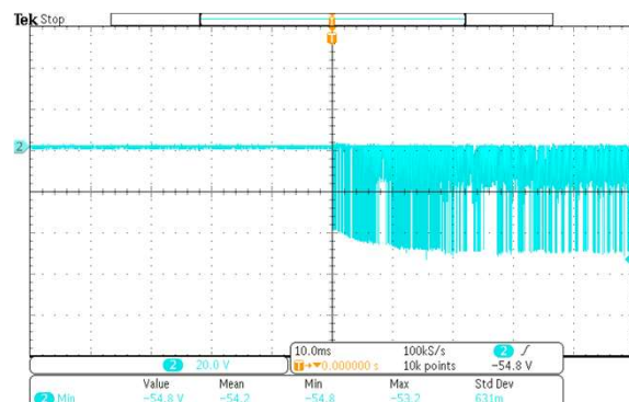
264Vac Turn On Vrr(min) : 54.8V
