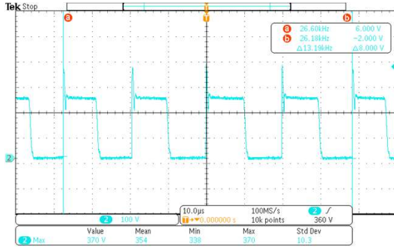
90Vac Full Load Vds(max) : 370V
