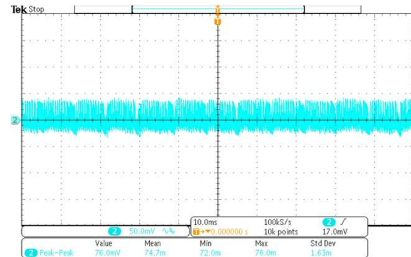
230Vac Full Load Noise: 76mV
