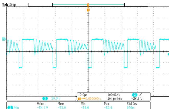
264Vac Full Load Vrr(min) : 54V
