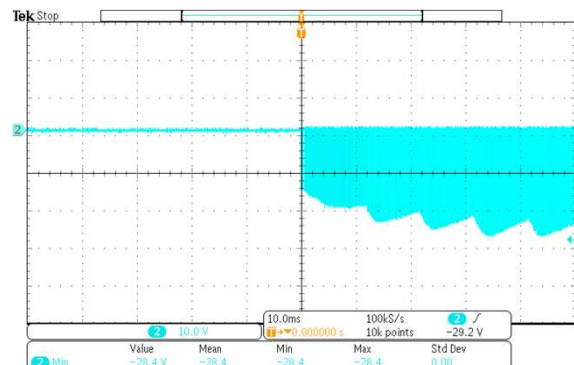
90Vac Turn On Vrr(min) : 28.4V
