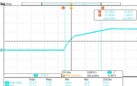
264Vac Rise Time: 26.8mS
