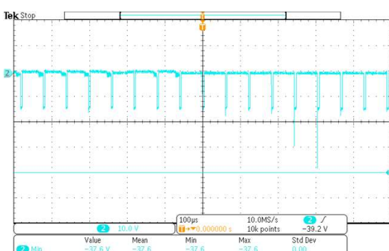
90Vac Operating short Vrr(min) : 37.6V
