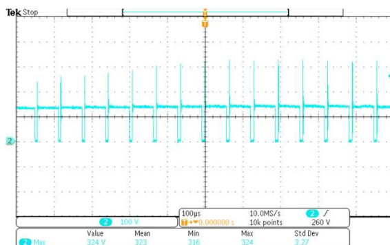
90Vac Operating Short Vds(max) : 324V
