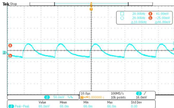
90Vac Full Load Ripple: 66mV
