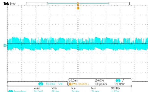
90Vac Full Load Noise: 78mV
