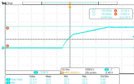
230Vac Full Load overshoot: 12.3V
