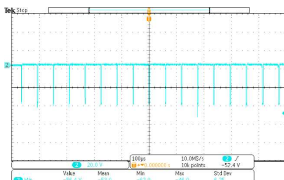
264Vac Operating short Vrr(min) : 56.4V
