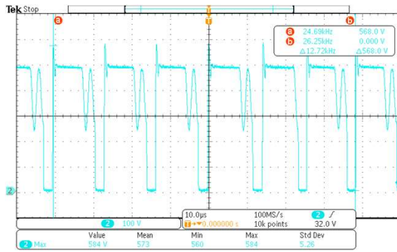
264Vac Full Load Vds(max) : 584V
