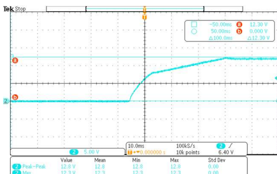
264Vac Full Load overshoot: 12.3V
