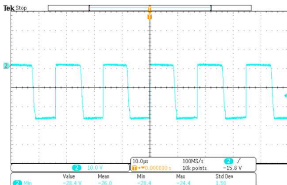
90Vac Full Load Vrr(min) : 28.4V
