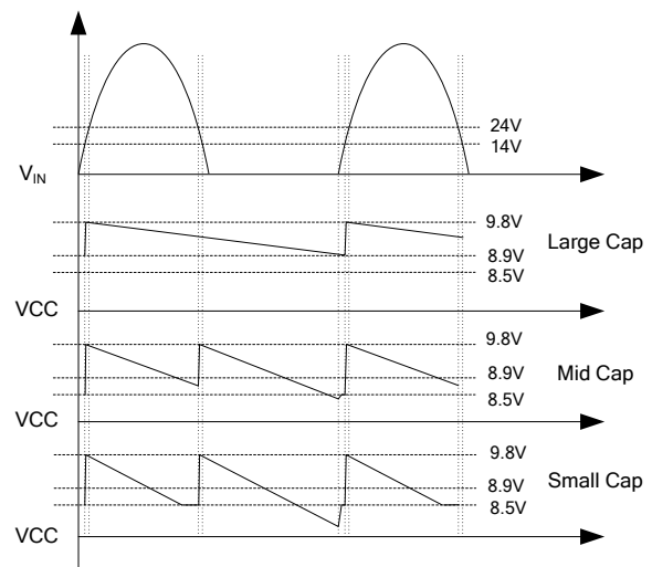
Figure 3: VCC Voltage in Different Capacitance
