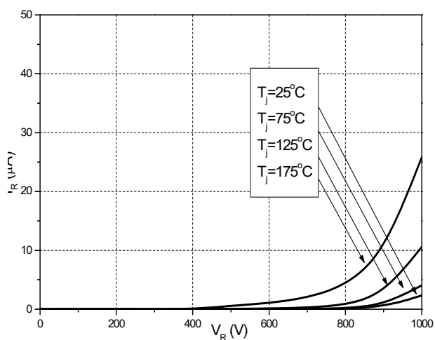
Figure 2. Reverse Characteristics
