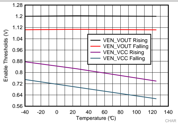
Figure 8. Enable Thresholds
