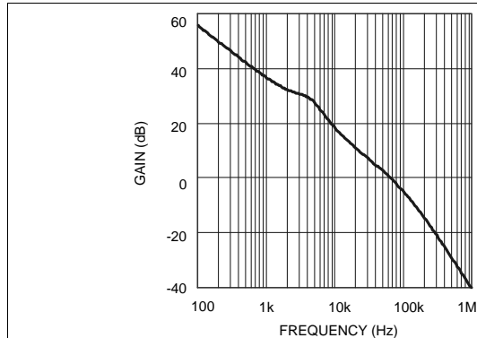
Figure 37. Gain vs Frequency
