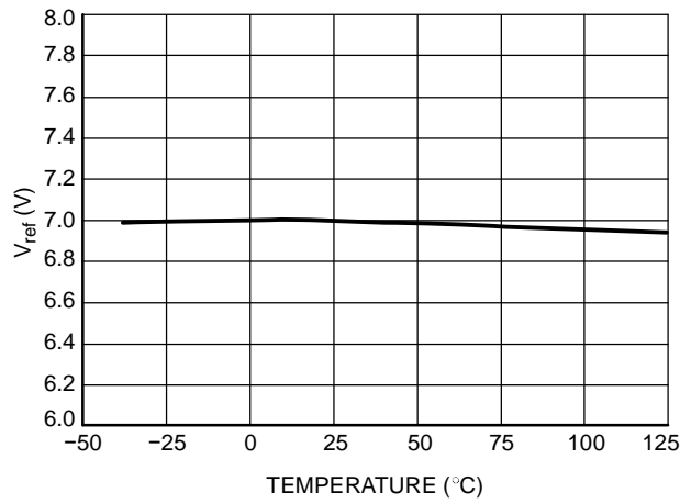
Figure 11. OVP internal Reference Level versus Temperature
