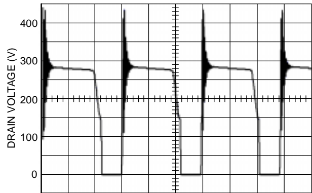
Figure 19. The NCP1207A Operates in Borderline / Critical Operation
