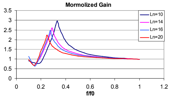
Figure 9. L_n impacts on LLC converter voltage gain
