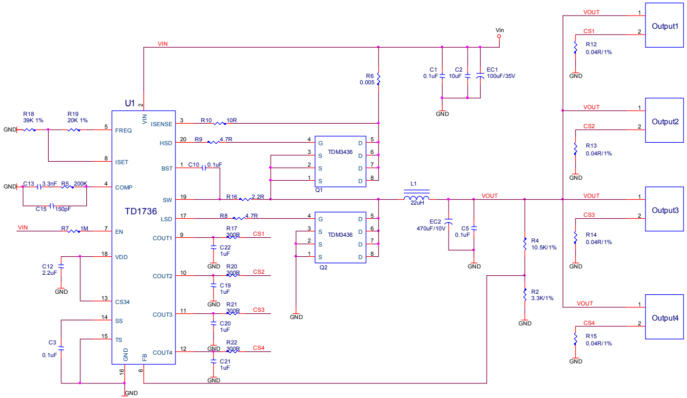
Fig3 4-outputs with OCP(CS1~4) and CC(CS1+CS2+CS3+CS4)
