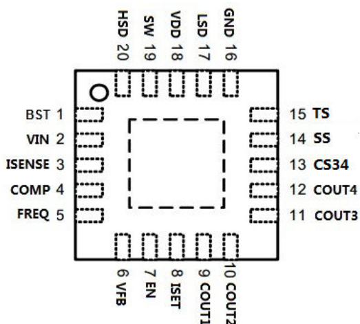
Figure1 Pin Configuration of TD1736(Top View)
