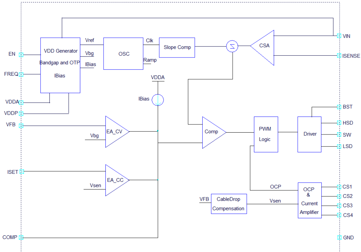
Figure 2 Function Block Diagram of TD1736
