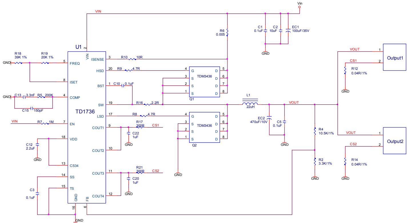
Fig4 2-outputs with OCP and CC(CS1+CS2)
