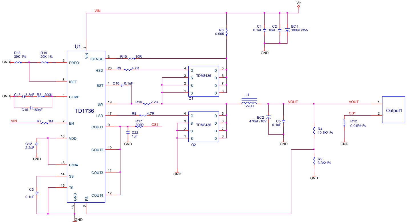
Fig5 1 output with CC.
