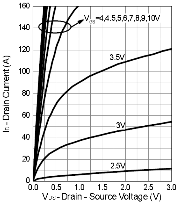
Output Characteristics
