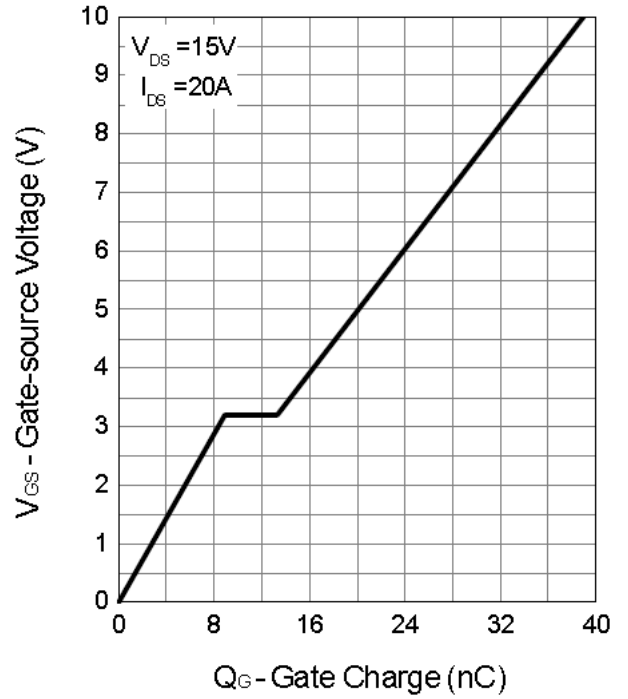
Gate Charge
