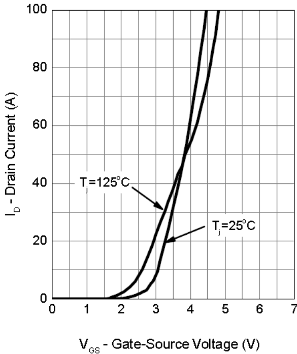
Transfer Characteristics
