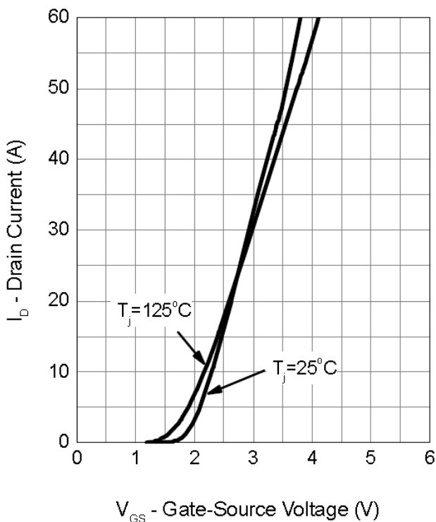
Transfer Characteristics
