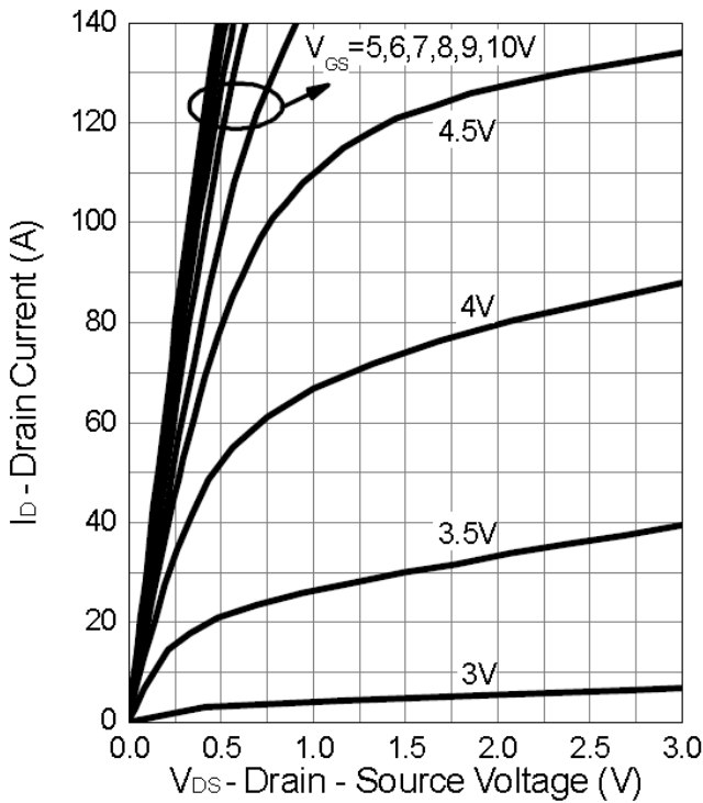
Output Characteristics
