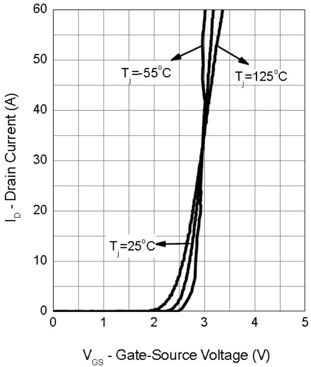
Transfer Characteristics
