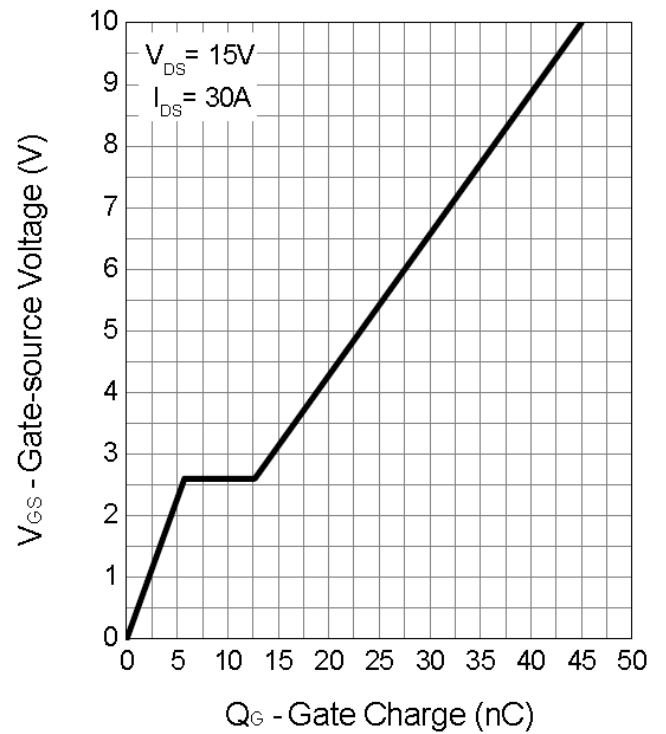
Gate Charge
