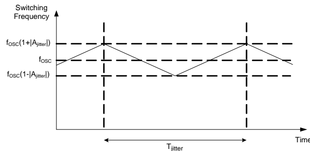
Figure 3: Frequency Jittering
