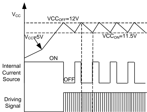
Figure 5: Self-Power Supply
