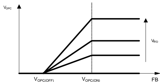
Figure 7: Compensation Current vs. FB and B/O Voltage
