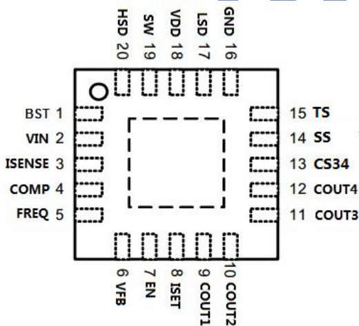
Figure1 Pin Configuration of TD1736(Top View)
