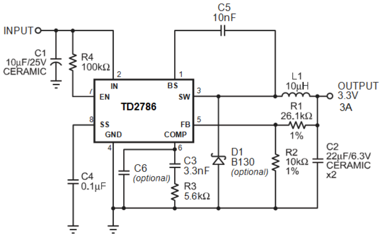
Fig13. TD2786 with 3.3V Output, 22µF/6.3V Ceramic Output Capacitor
