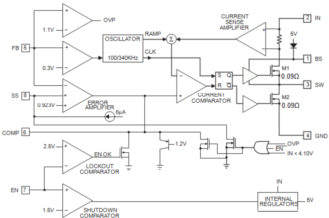
Figure 3 Function Block Diagram of TD2786
