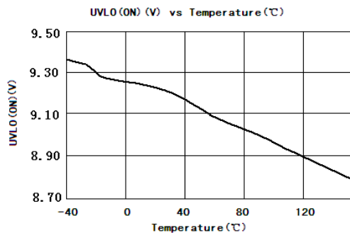
Figure 6.3 UVLO(ON)(V) vs Temperature(°C)
