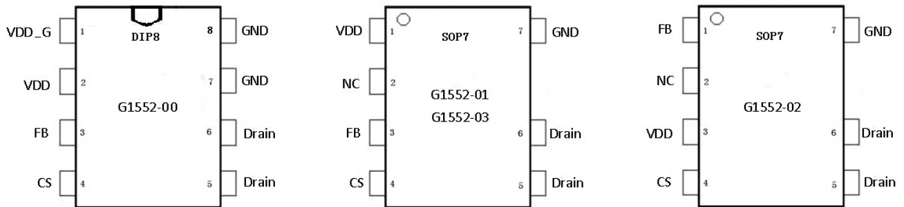
Pin Configuration: G1552 Series
