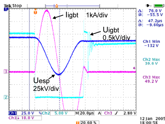
Fig. 10 ESP and IGBT voltage and IGBT current during a normal pulse.
