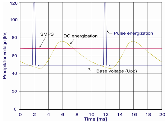
Fig. 2 Waveform of the output voltage
