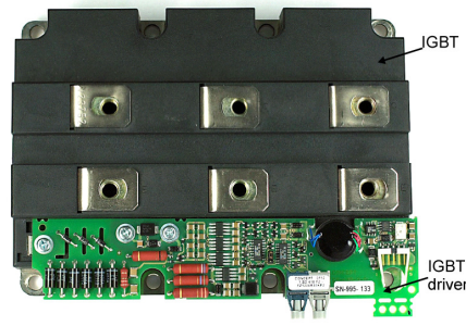
Fig. 9 1200A/3300 V IGBT used as switch
