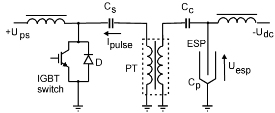
Fig. 3 Simplified main circuit of a Coromax pulse system
