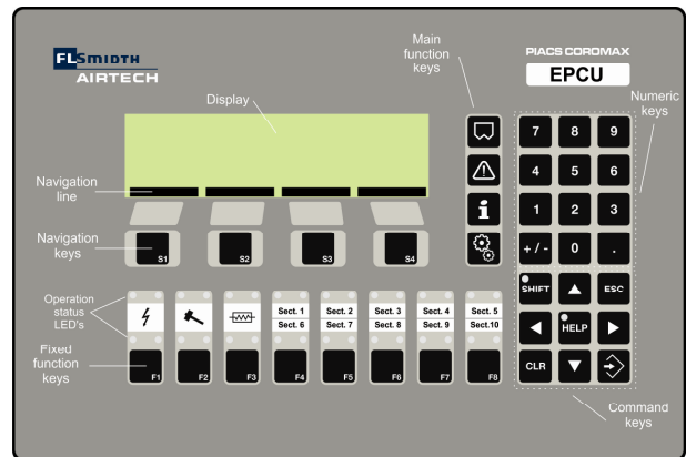
Fig. 6 Front panel of the control system
