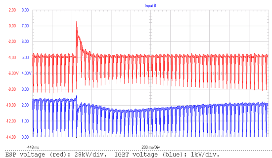
Fig. 12 ESP voltage and IGBT voltage at normal repetitive operation.
