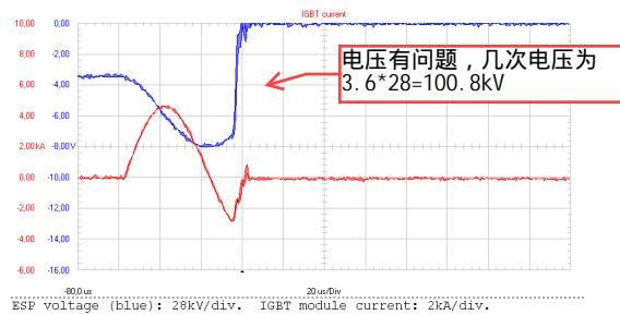
Fig. 11 ESP voltage and IGBT current during a pulse spark.
