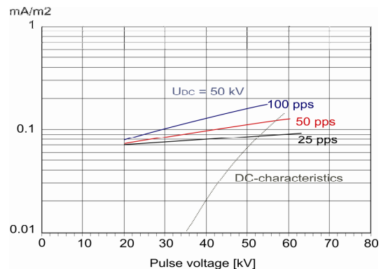
Fig. 13 Pulse and DC I-V characteristics
