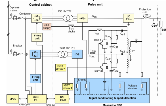
Fig. 5 Block diagram of the COROMAX
