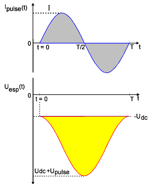
Fig. 4. Waveforms during a normal high voltage pulse
