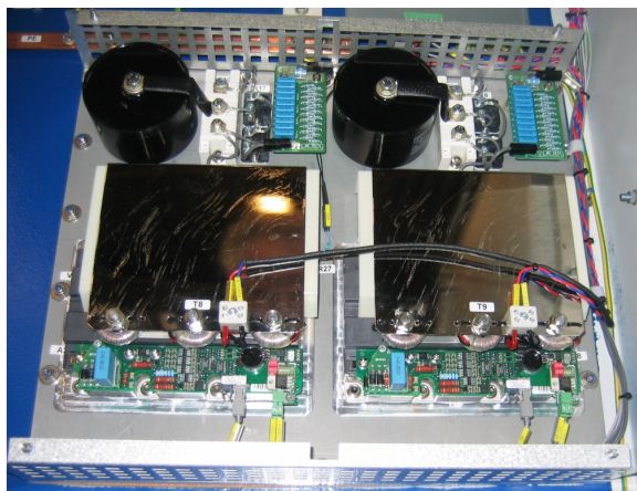
Fig. 8 IGBTs mounted in LVJB
