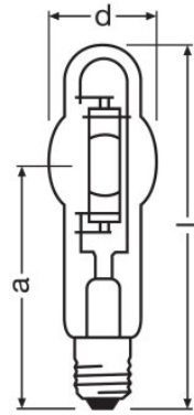
HQI-BT 400 W/D PRO
