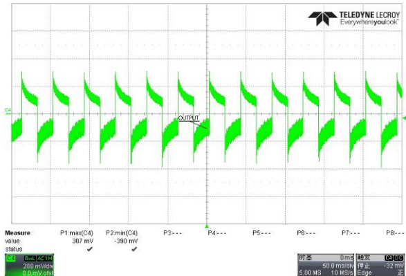
Fig. 12 Dynamic waveform @264Vac input
