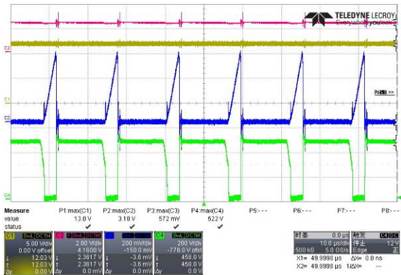
Fig. 24 CS,FB,Vdd&Vds wave form @264Vac; full load
