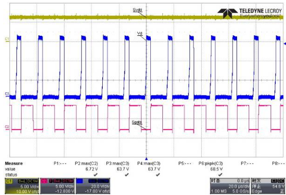
Fig. 28 Synchronous rectification Sgate, Svdd & Vd waveform @264Vac; full load
