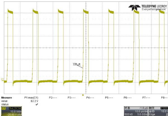
Fig. 32 Vds_sr normal wave form @264Vac; full load
