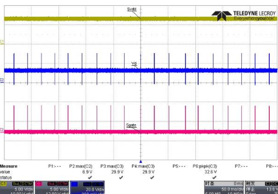
Fig. 25 Synchronous rectification Sgate, Svdd & Vd wave form @90Vac; no load
