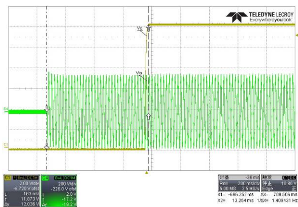
Fig. 14 Turn on delay waveform @240Vac; full load
