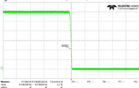
Fig. 8 Overshoot waveform @264Vac; no load
