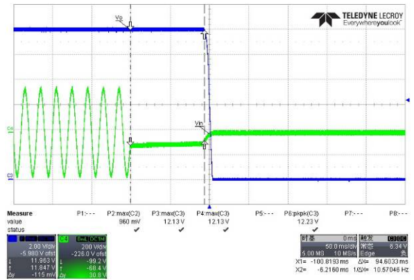
Fig. 16 Hold up time waveform @240Vac; full load
