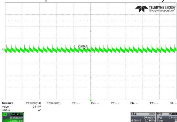
Fig. 1 R&N waveform@90Vac; no load
