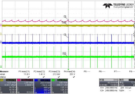
Fig. 21 CS,FB,Vdd&Vds wave form @90Vac; no load
