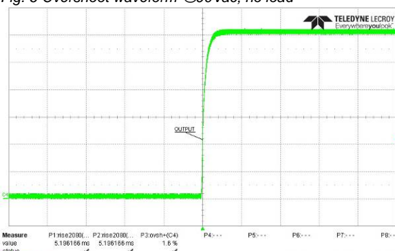
Fig. 6 Overshoot waveform @90Vac; no load
