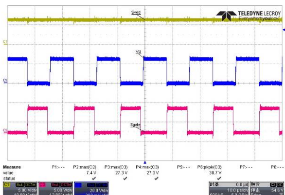
Fig. 26 Synchronous rectification Sgate, Svdd & Vd wave form @90Vac; full load
