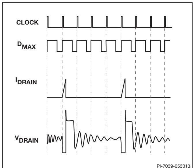
Figure 9. Operation at Very Light Load.
