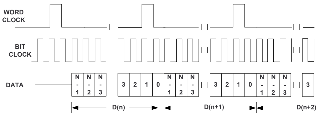
图 38. Timing Diagram for Mono PCM Mode with ASI_OFFSET1=2
