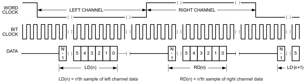
图 28. Timing Diagram for I 2 S Mode with ASI_OFFSET1 = 2
