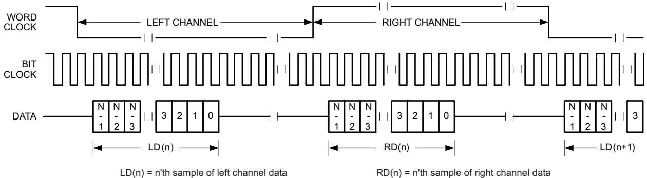
图 29. Timing Diagram for I 2 S Mode with ASI_OFFSET1 = 0 and Inverted Bit Clock
