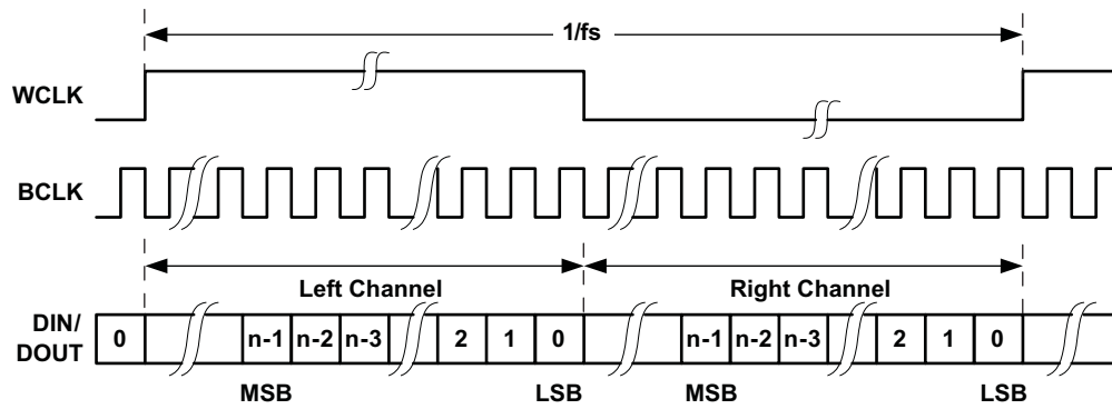
图 33. Timing Diagram for Right-Justified Mode
