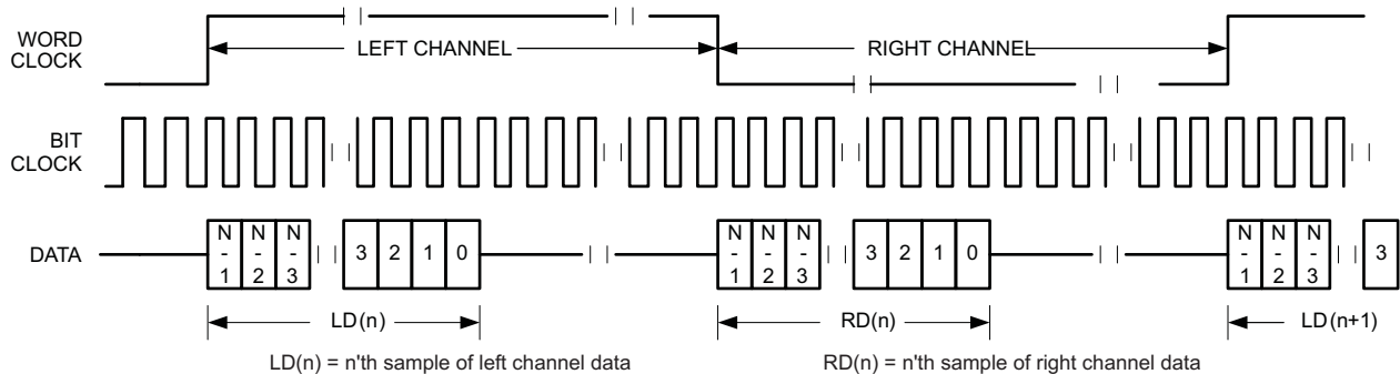
图 36. Timing Diagram for Left-Justified Mode with ASI_OFFSET1 = 0 and Inverted Bit Clock
