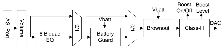
图 41. ROM Mode 1 Processing Block Diagram
