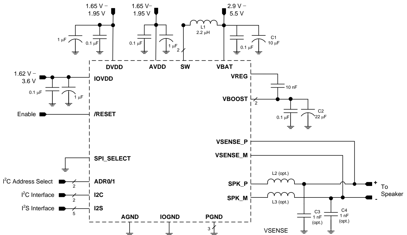
图 43. Typical Application - Digital Audio Input
