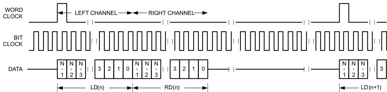
图 32. Timing Diagram for DSP Mode with ASI_OFFSET1=0 and Inverted Bit Clock
