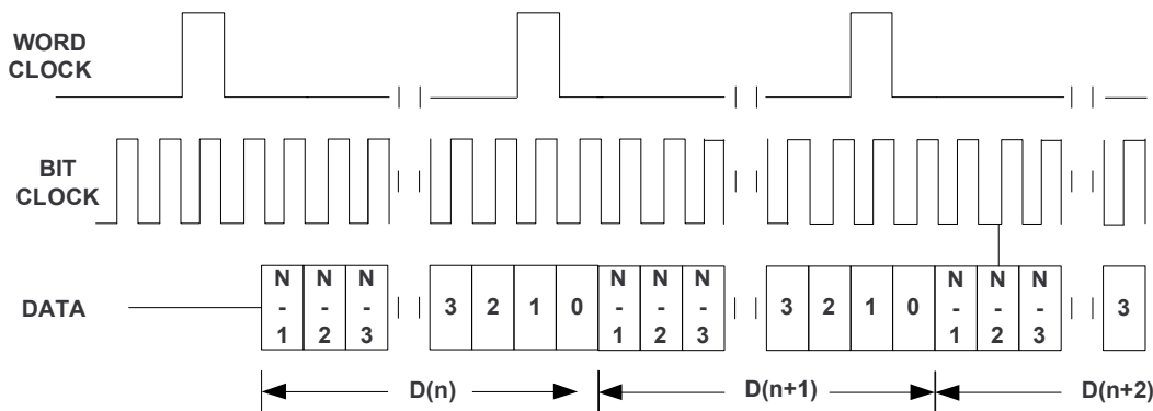
图 39. Timing Diagram for Mono PCM Mode with ASI_OFFSET1=2 and Bit Clock Inverted
