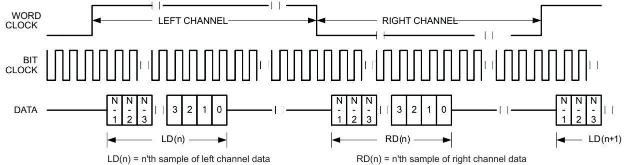
图 35. Timing Diagram for Light-Left Mode with ASI_OFFSET1 = 1
