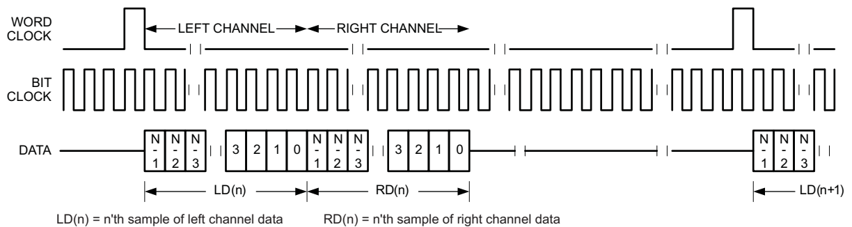
图 31. Timing Diagram for DSP Mode with ASI_OFFSET1=1
