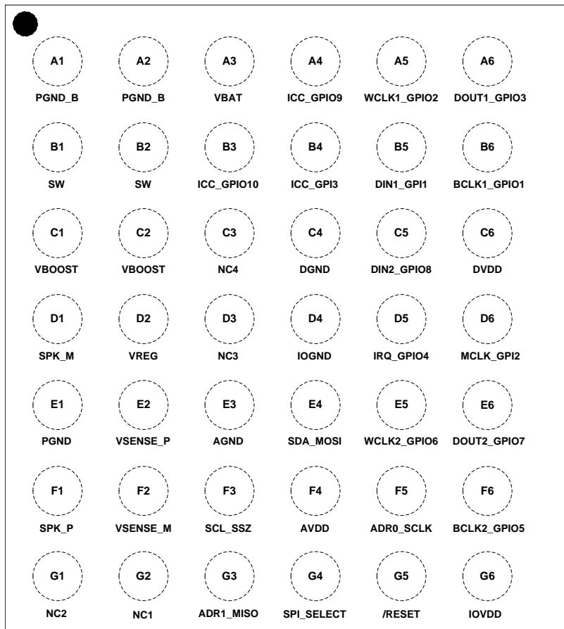
Pin Functions
