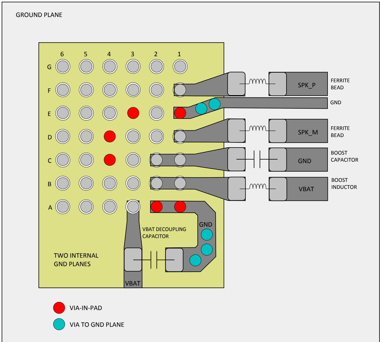
图 46. TAS2557 Board Layout
