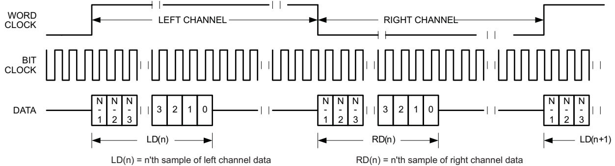
图 34. Timing Diagram for Left-Justified Mode
