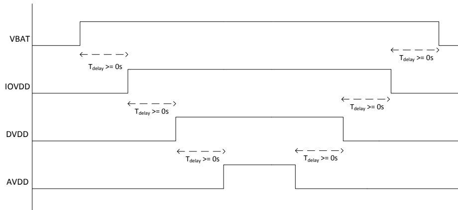
图 45. Power Supply Sequence for Power-Up and Power-Down
