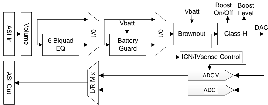
图 42. ROM Mode 2 Processing Block Diagram
