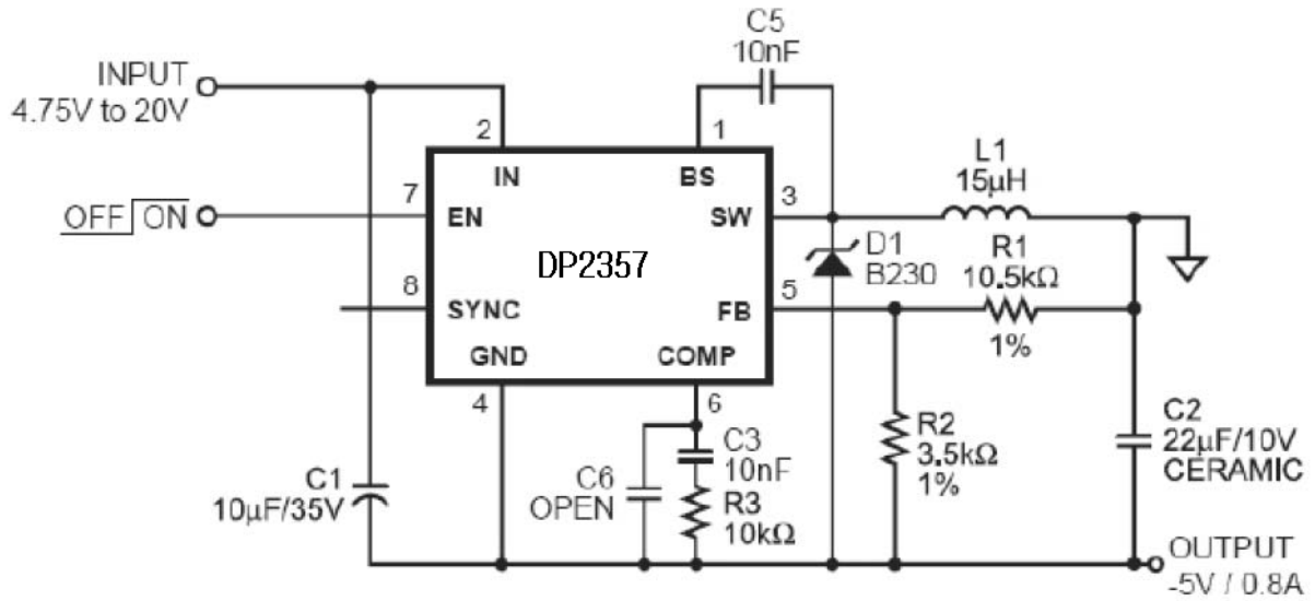
Figure 3—Application Circuit for -5V Supply
