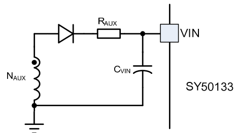
Fig. 8 Filter resistor R_{AUX}
