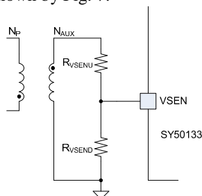
Fig. 7 Cable Compensation
