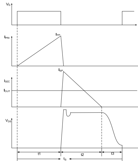
Fig.9 switching waveforms
