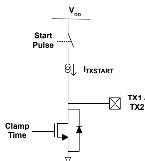
Figure 5: Output Stage
