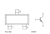
Fig. 1 Simplified outline (SOT23) and symbol. Q7:PMBT2222
