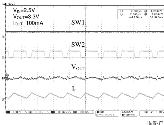
Fig. 19 Boost Operation
