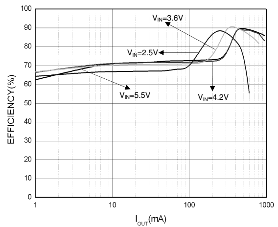
Fig.5 Efficiency vs. Output Current V_{OUT} = 3.3V (PSM Mode)
