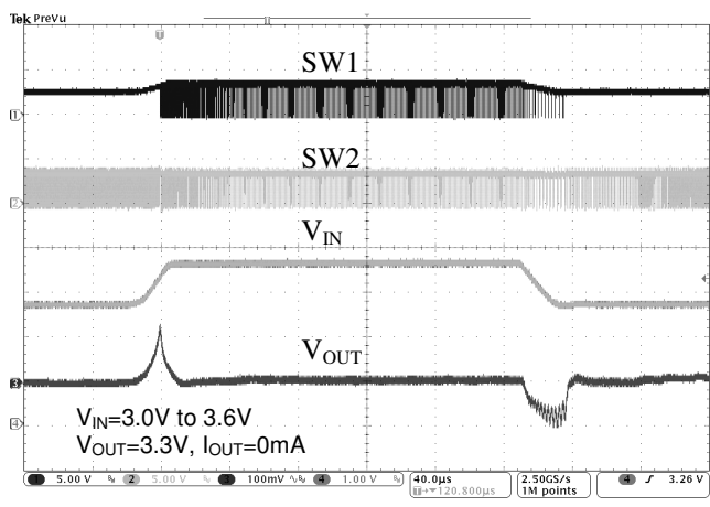
Fig. 14 Line transient (PWM mode)
