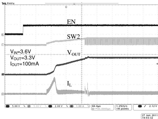
Fig.24 Start-up (PWM)
