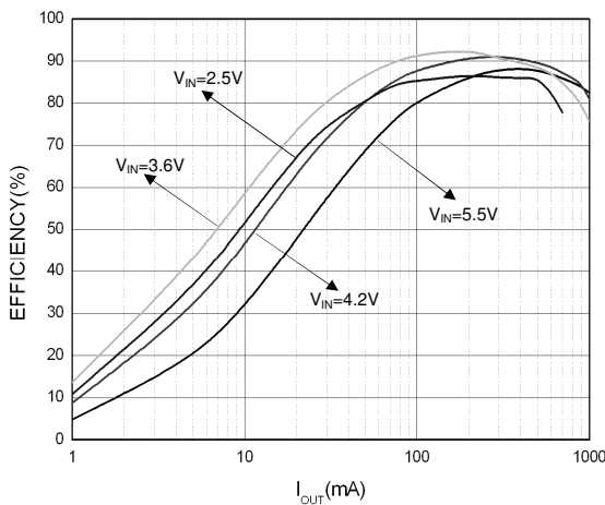
Fig.6 Efficiency vs. Output Current V_{OUT} = 2.8V (PWM Mode)
