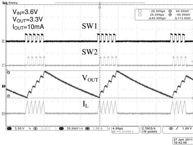
Fig.20 PSM Operation
