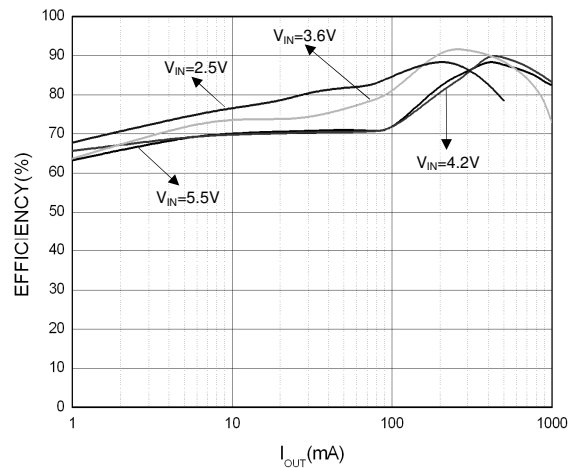
Fig.7 Efficiency vs. Output Current V_{OUT} = 2.8V (PSM Mode)
