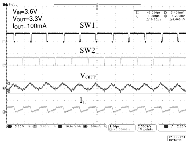
Fig. 18 Buck-Boost Operation
