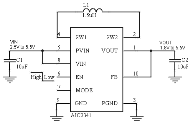
Fig.1 Application Circuit
