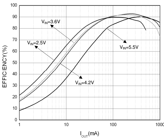
Fig.4 Efficiency vs. Output Current V_{OUT} = 3.3V (PWM Mode)
