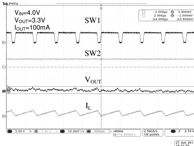
Fig. 17. Buck operation
