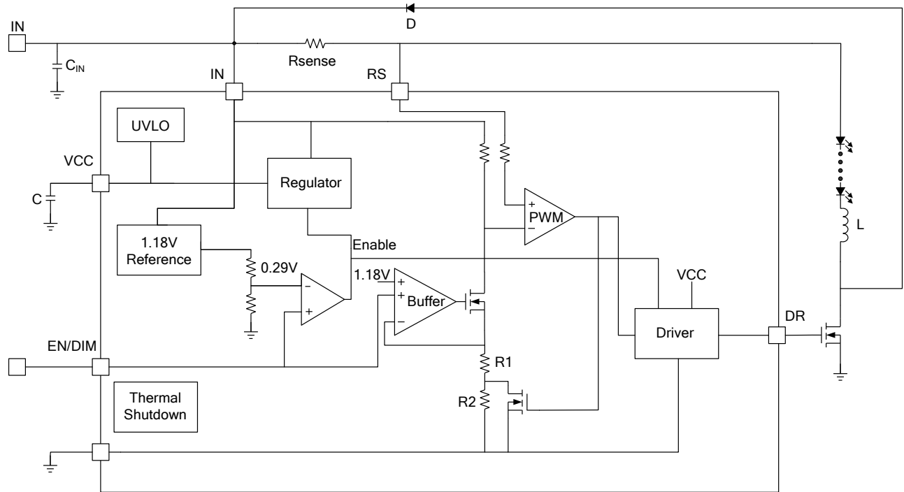
Figure 1—FM76651 Functional Block Diagram
