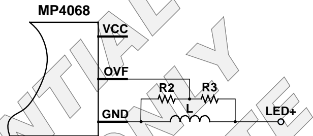
FIGURE 7. Feedback Resistor Connection
