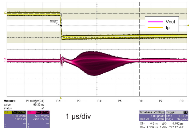
Figure 9: dv/dt
