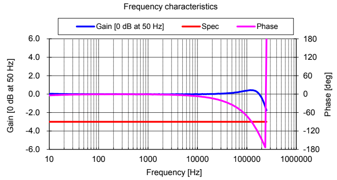
Figure 7: Frequency response
