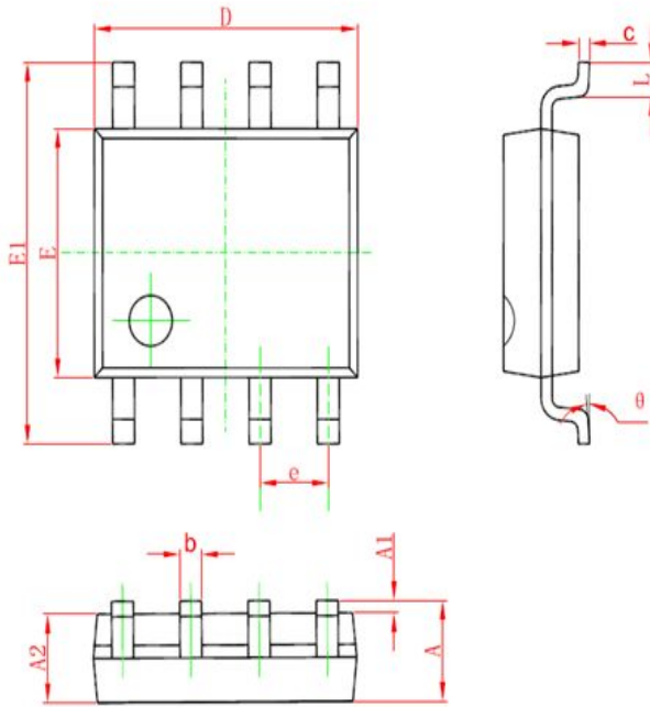
SOP8 PACKAGE OUTLINE DIMENSIONS
