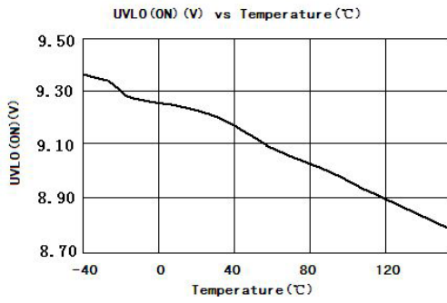
Figure 6.3 UVLO(ON)(V) vs Temperature(°C)
