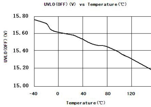
Figure 6.2 UVLO(OFF)(V) vs Temperature(°C)
