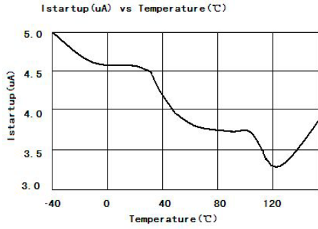
Figure 6.1 Istartup(μA) vs Temperature(°C)
