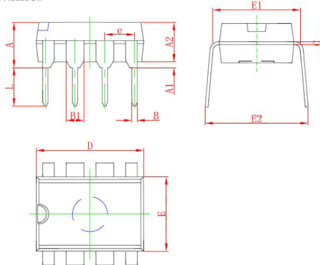
8-Pin Plastic DIP
