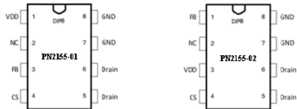
Pin Configuration: PN2155 Series
