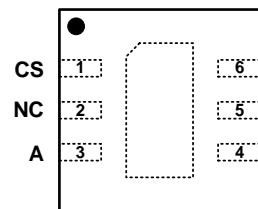
DFN- 2mmx2mm-6L
