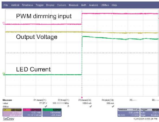
Fig. 8a: Rise time of LED Current at 80V output (5 \mu s/div)
