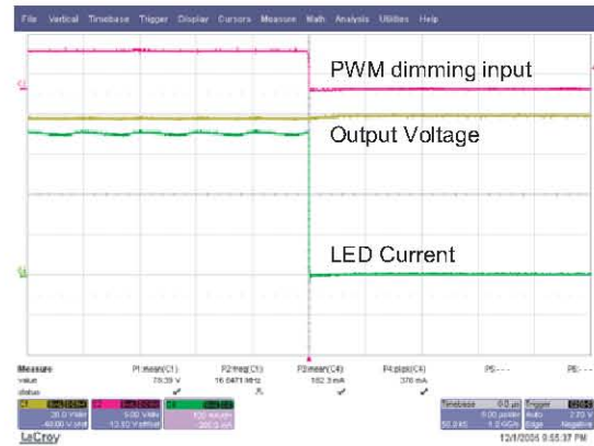
Fig. 8b: Fall time of LED Current at 80V output (5 \mu s/div)
