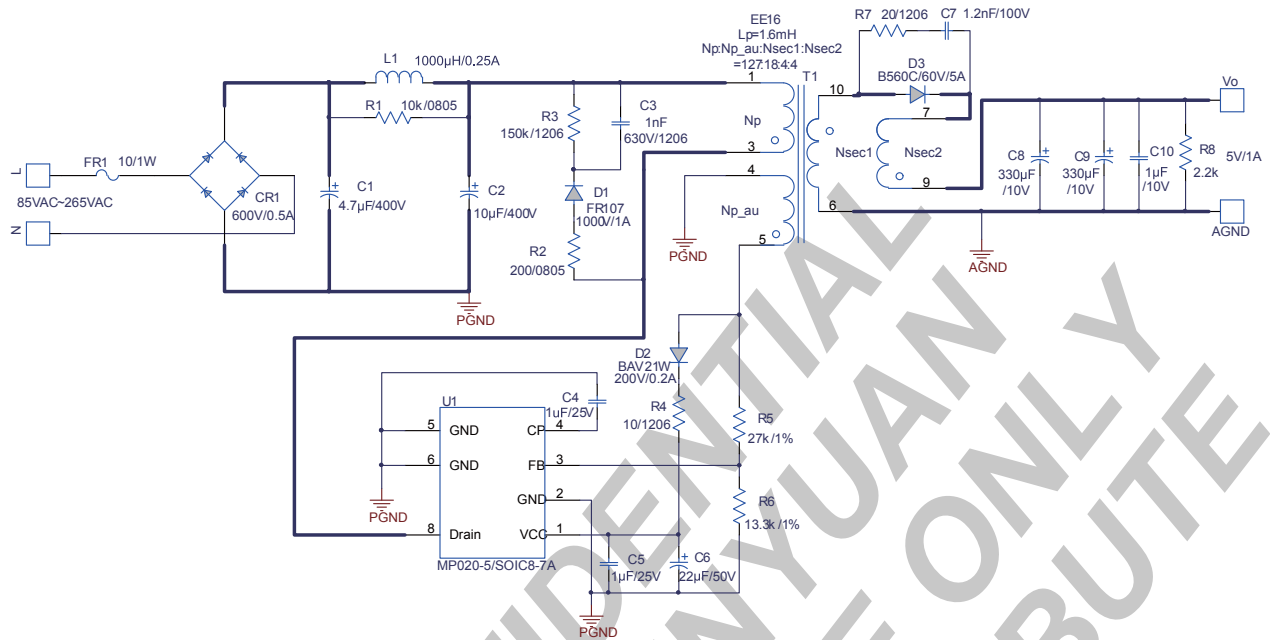
Figure 14: Typical Application, 5V/1A
