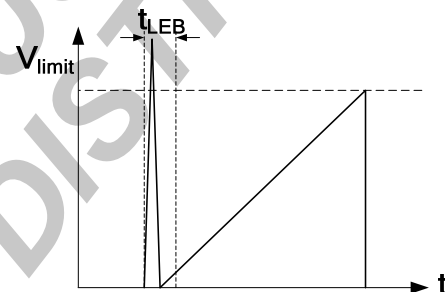
Figure 7: Leading-Edge Blanking
