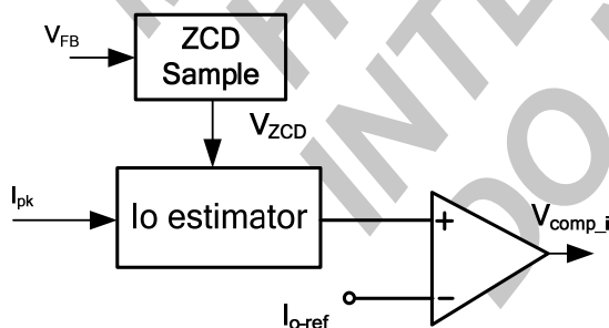
Figure 6: CC Control Loop
