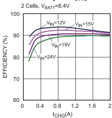
Efficiency vs. I_CHG
