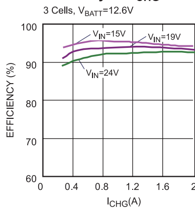
Efficiency vs. I_CHG
