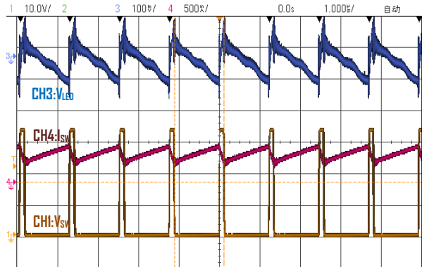
Switching Waveform VIN=3.6V, 10LEDs, IOUT= 40mA
