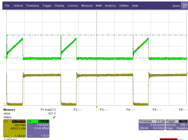
Figure 21 – 300 VAC / 63 Hz, 36 V LED String. Measured V_{DRAIN} Stress: 621 V. Ch1: V_{DRAIN} , 200 V / div. Ch4: I_{DRAIN} , 01 A / div., 5 µs / div.
