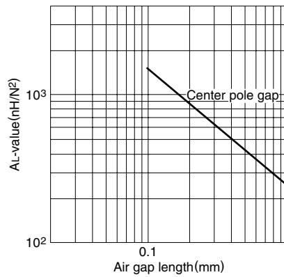
AL-value vs. Air gap length for PC40RM14 core (Typical)
