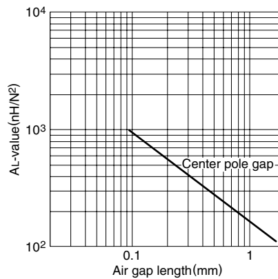
AL-value vs. Air gap length for PC40EER35 core (Typical)
