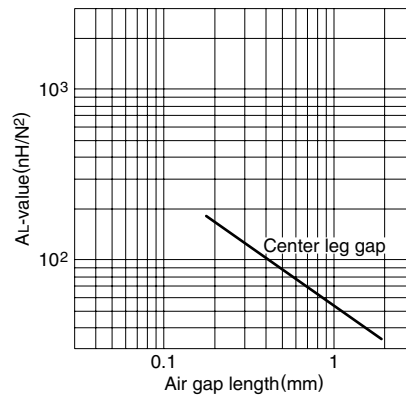
AL-value vs. Air gap length for PC40EE20/20/5 core (Typical)
