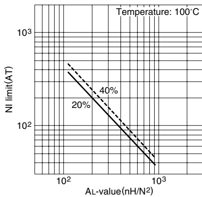
NI limit vs. AL-value for PC40EER35 gapped core (Typical)
