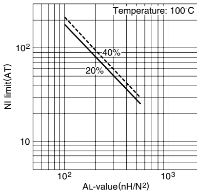
NI limit vs. AL-value for PC40ETD24 gapped core (Typical)
