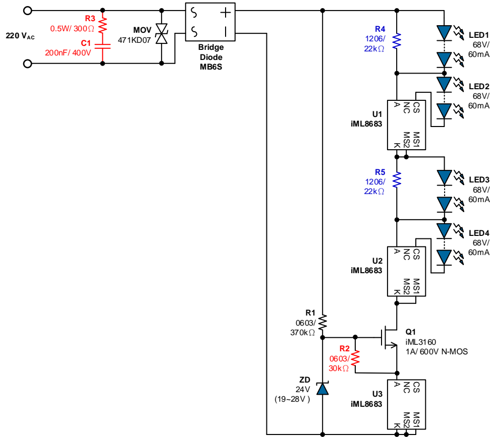
220VAC System
