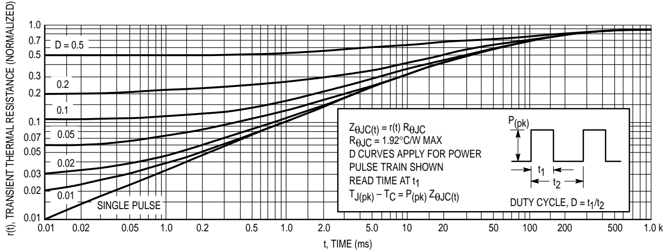
Figure 4. Thermal Response
