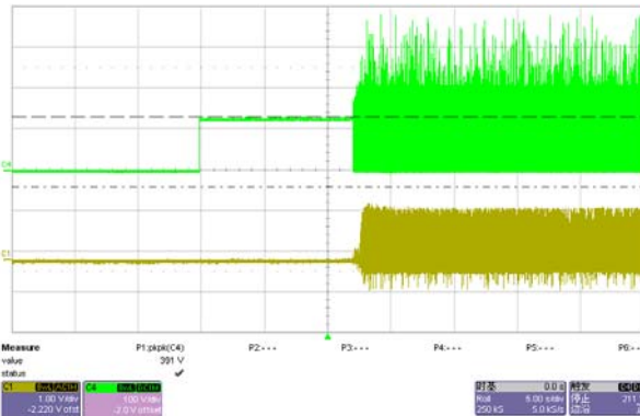
Fig. 12 Start, Vds waveform@90 Vac/60Hz, full load
