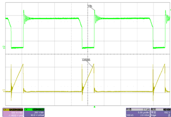
Fig. 17 Normal, Vds&Ids waveform@264 Vac/60Hz, full load
