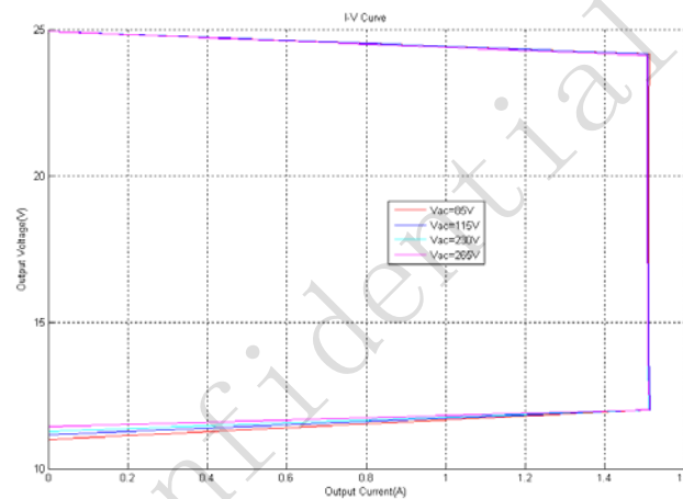
Fig. 4 CC/CV Characteristics
