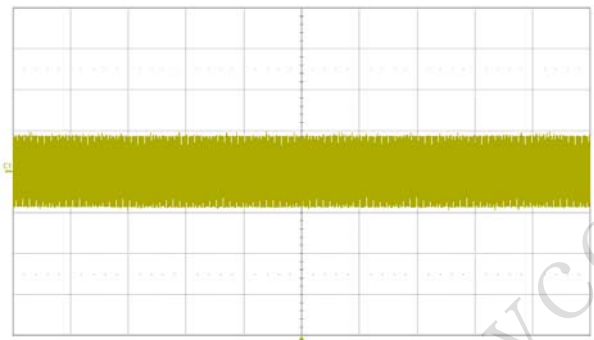
Fig. 6 Measured ripple & noise waveform @90Vac/60Hz, full load
