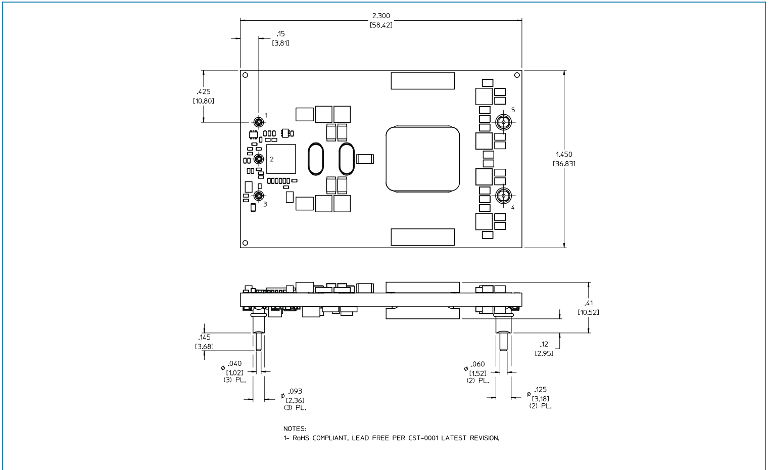
Figure 31 — IBC outline drawing
