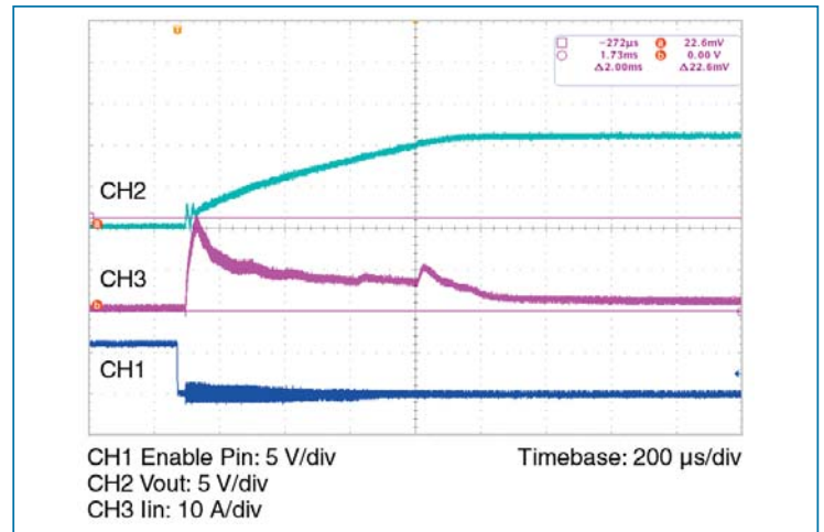
Figure 4 — Inrush current at nominal line full load; 10 A/div
