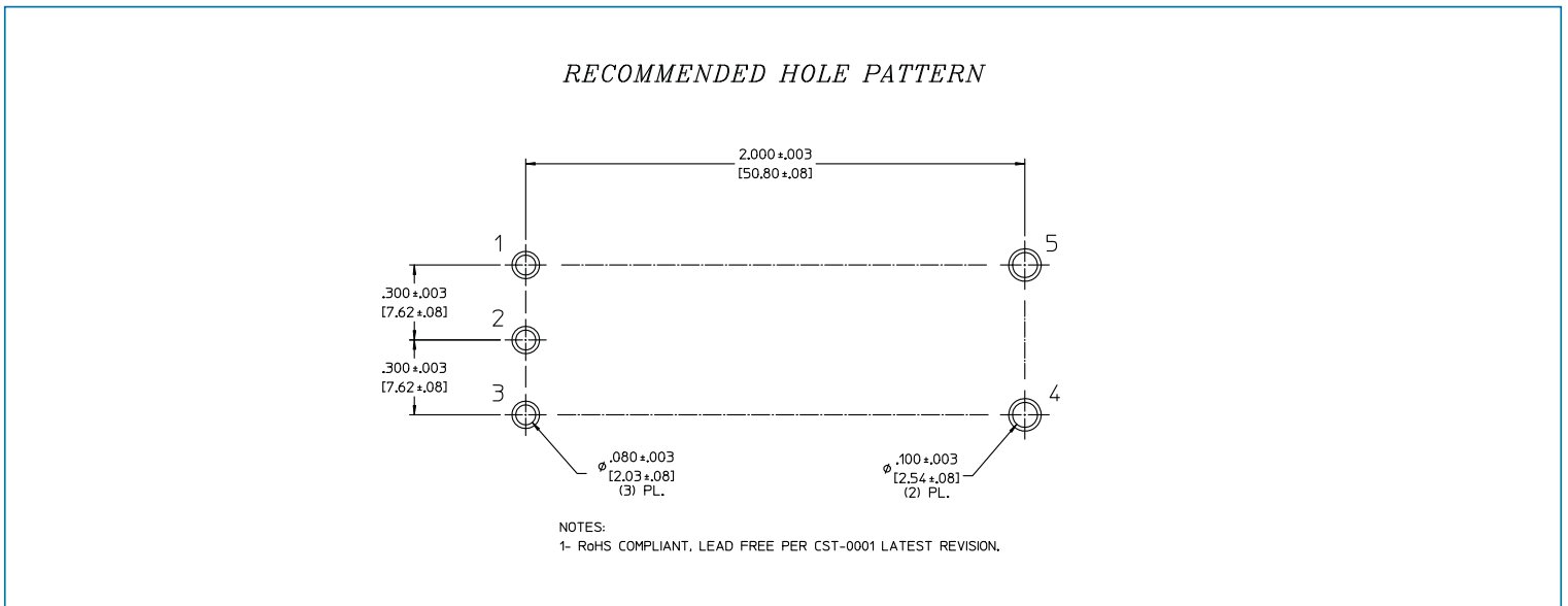
Figure 32 — IBC PCB recommended hole pattern
