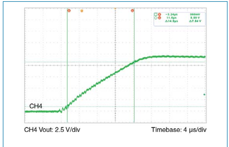
Figure 8 — Output voltage rise time at nominal line, full load
