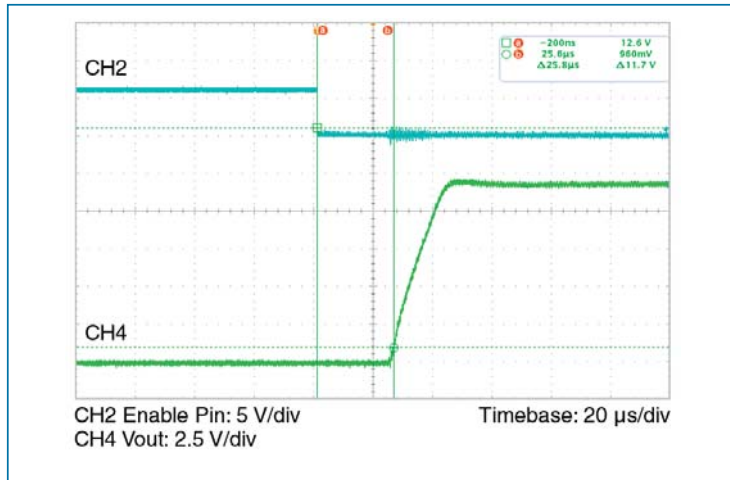
Figure 7 — Turn on delay time; Enable turn on delay at nominal line, full load
