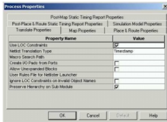
Figure 5.3.7 Process Properties
