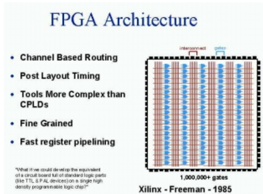
Figure 1.4 FPGA Architecture
