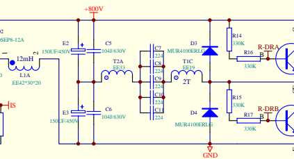
BUCK +800V降至+400V
