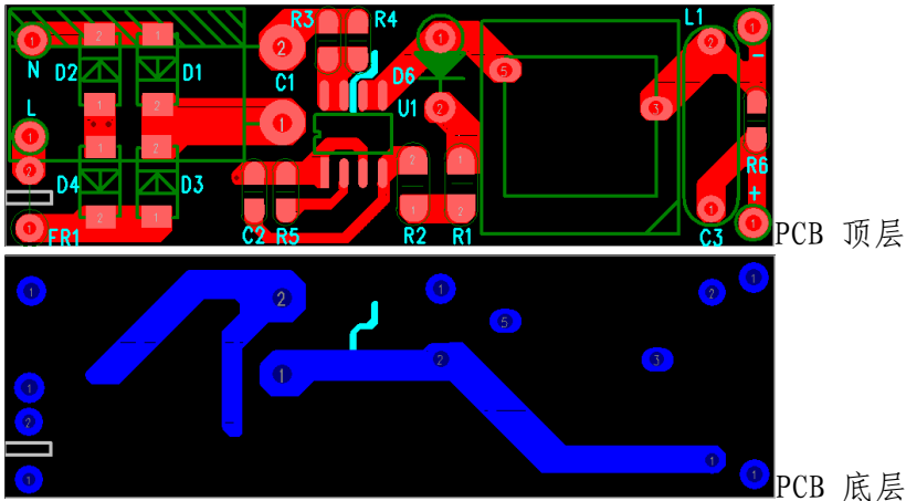
PCB Layout 51mm*16mm
