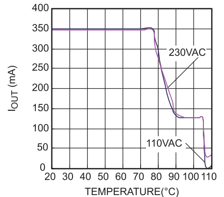
NTC Curve
