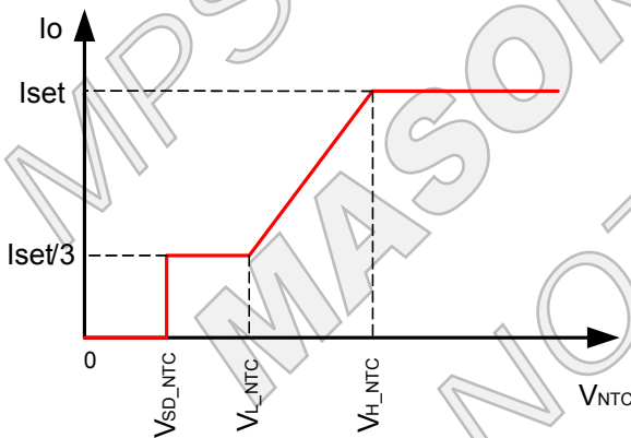
Figure 11: NTC Curve
